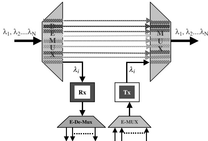
Figure 19.7 Substrate multiplexing makes efficient use of wavelength bandwidth by aggregating/grouping data at OADM nodes.
