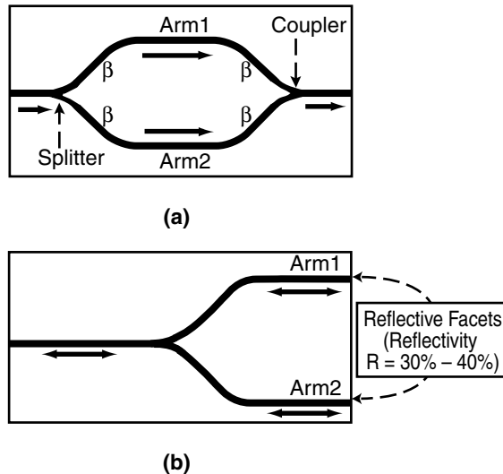
Figure 21.2 (a) Mach–Zehnder interferometer; (b) Michelson interferometer.
