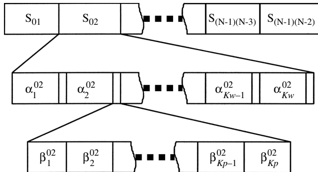
Figure 18.4 The encoding formate of SAPP solutions.
