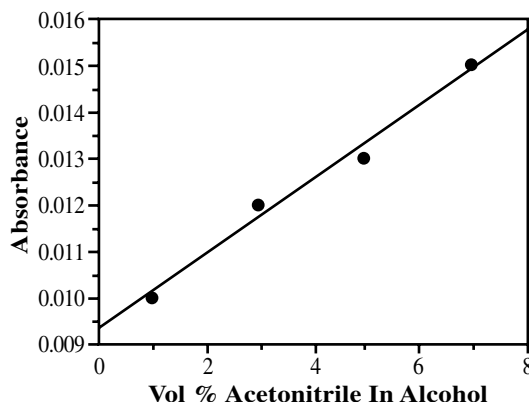
Figure 20.19 Calibration curve for acetonitrile in alcohol. (From T. Iqbal et al., Optics Lett. , 16, 1611, 1991. With permission.)
