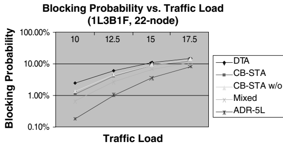
Figure 11.11 (continued) Blocking probability vs. traffic load with different percentages of switching types in the 16-node and 22-node networks. CB-STA w/o is a CB-STA tunnel allocation without the makeup process. (P.H. Ho and H.T. Mouftah, Routing and wavelength assignment with multi-granularity traffic in optical networks, IEEE, Aug. 2002. With permission.)
