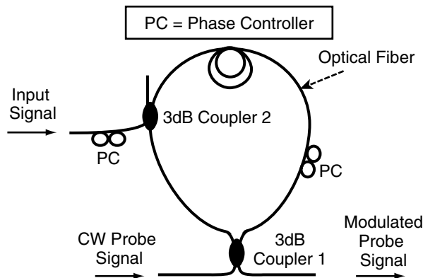
Figure 21.4 Nonlinear-optical loop mirror using optical fiber.
