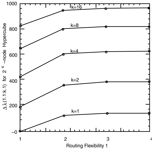
Figure 12.12 The incremental throughput gain \lambda(1, 1; k, l) , for k = 1, 2, 4, 8, 16 and l = 1, 2, 3, 4 , for a 2^6 -node hypercube network with P_{succ} = 0.8 .
