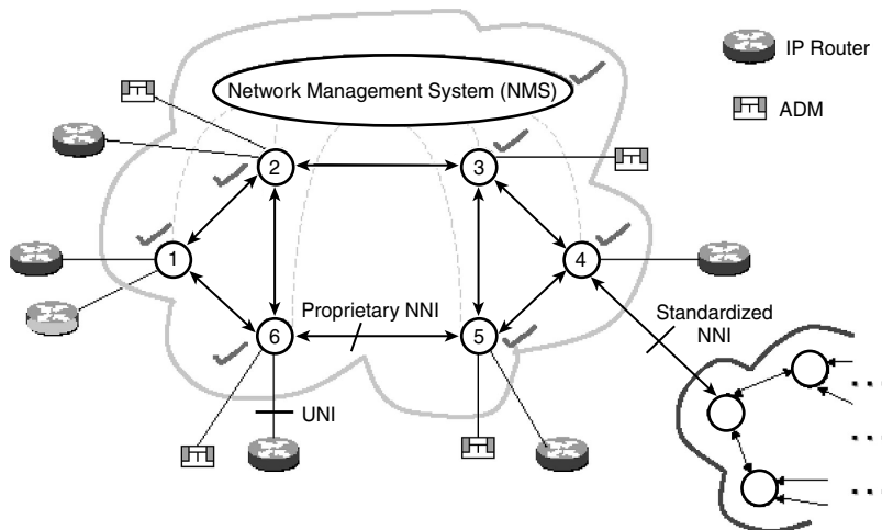
Figure 1.15 Network management system for IP-over-WDM networks.
