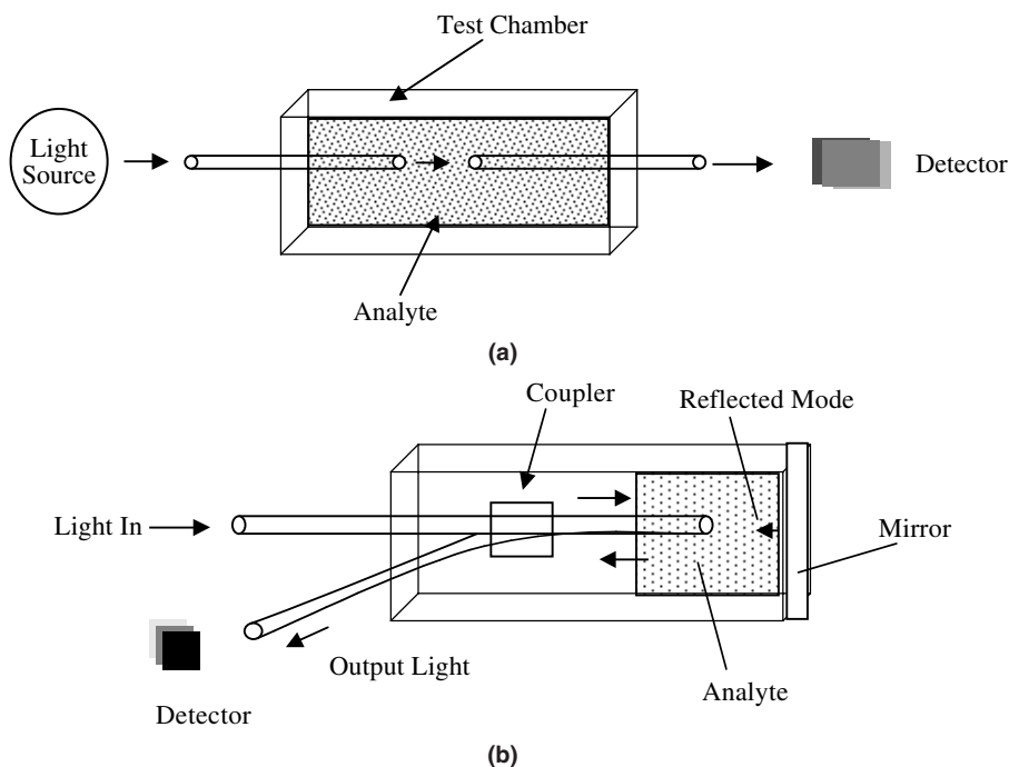
Figure 20.22 (a) Light interacting directly with the analyte via an optical fiber. (b) Light interacting indirectly with the analyte via an optical fiber.
