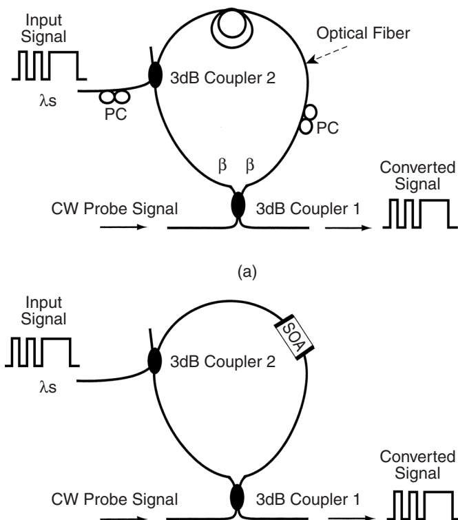
Figure 21.7 NOLM wavelength converters: (a) fiber loop; (b) SOA as the nonlinear medium.
