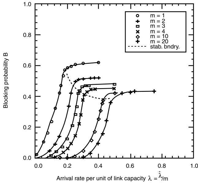
Figure 12.4 Performance results for the VCD protocol, illustrating the blocking probability B as a function of the normalized arrival rate per unit of link capacity \hat{\lambda}/m for an 8 \times 8 MS network and several values of m . The dashed lines correspond to the stability boundary.
