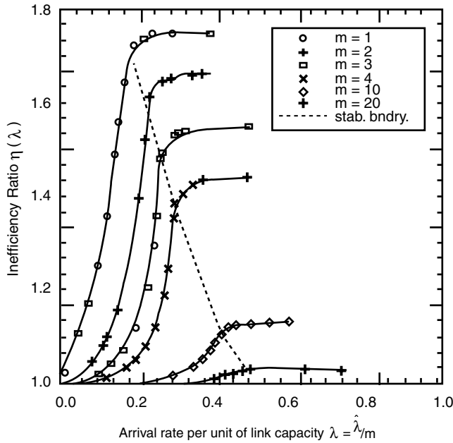
Figure 12.5 Performance results for the VCD protocol, illustrating the inefficiency ratio \eta(\lambda) as a function of the normalized arrival rate per unit of link capacity \lambda = \hat{\lambda}/m , for an 8 \times 8 MS network and several values of m . The dashed lines correspond to the stability boundary.
