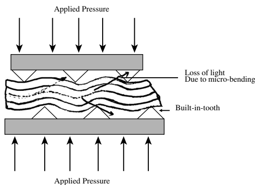
Figure 20.14 Mechanism of light loss due to micro-bending in an optical fiber.
