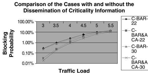
Figure 14.6 Comparison of the cases with and without the dissemination of criticality information. C-BAR-22 and C-BAR-30 are the cases without the criticality information dissemination. (P.H. Ho and H.T Mouftah, in Optical Networks — Architecture and Survivability , Kluwer Academic Publishers, Norwell, MA, pp. 88–103, 2003. With permission.)
